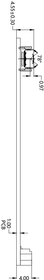
SIDE VIEW
