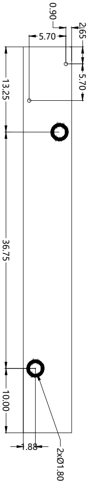
BOTTOM VIEW
