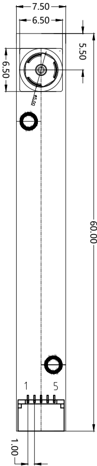
TOP VIEW
